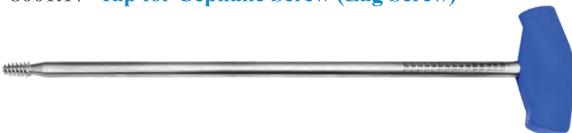
8001.17 Tap for Cephalic Screw (Lag Screw)
