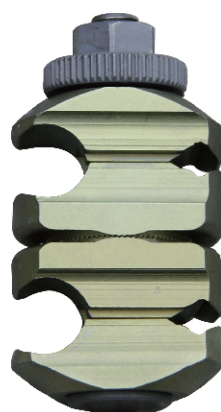
Pin to Rod Coupling (Large) EF345 - Aluminium EF348 - Titanium for Ø5-6mm pins/Ø11mm rods
